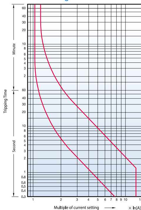
Hot starting
